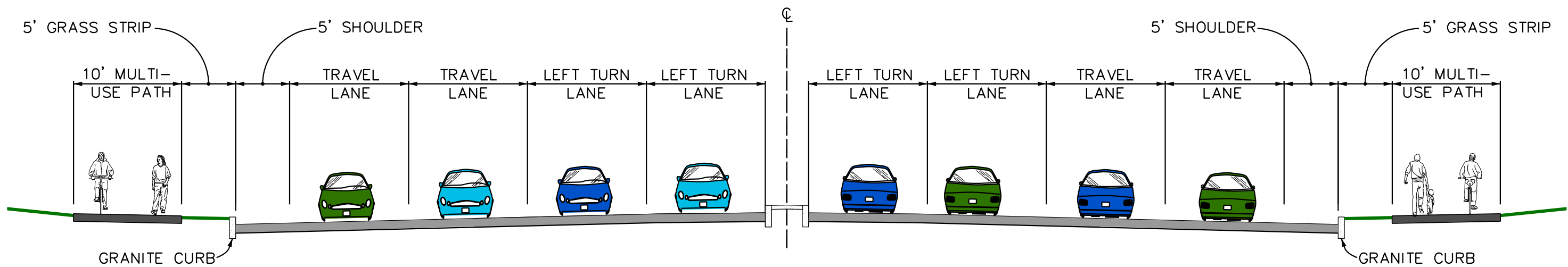
LOUDON ROAD - TYPICAL SECTION
